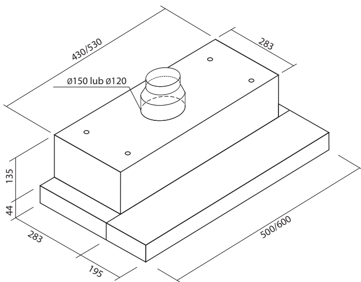
Okap AMADIS/AMADIS GLASS
